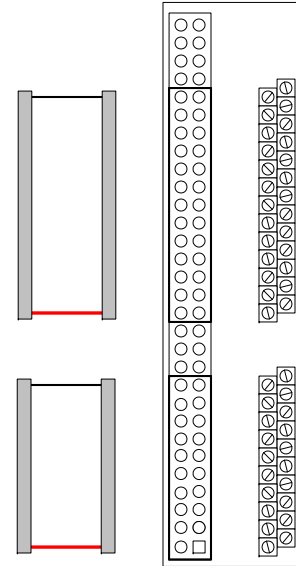
TB-20/26 CONFIGURATION
