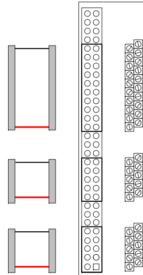
TB-10/10/20 CONFIGURATION
